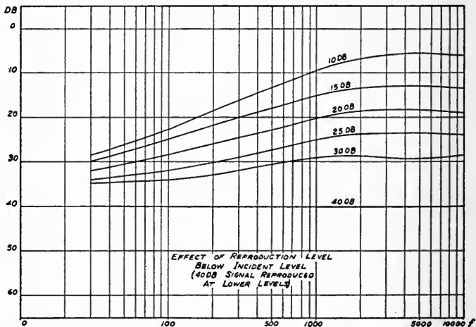
FIG. 3. Effect of reproduction level below incident level.
